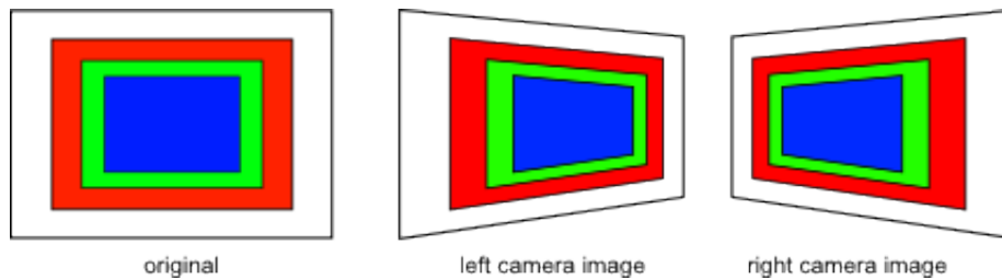
Figure 4: Keystone distortion
